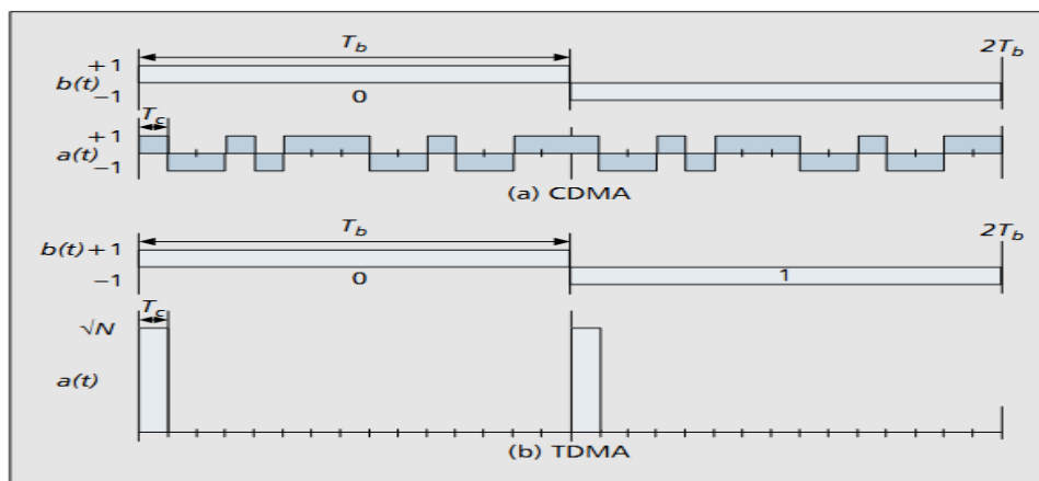
Figure 4: An example of the signature sequence for time domain multiple access: a) CDMA; b) TDMA
