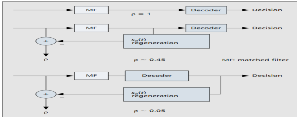
Figure 5: Interference cancellation factor
