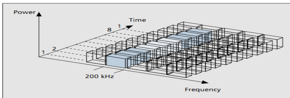
Figure 2: Physical channels in a GPRS system
